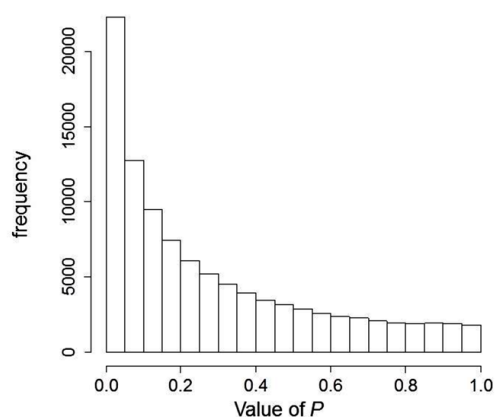
Figure 6 Distribution of 100,000 P values from tests like those in Fig 5, but with only 4 observations in each group, rather than 16. The calculated power of the tests is only 0.22 in this case, and it’s found, as expected, that 22% of the P values are equal to or less than 0.05.
